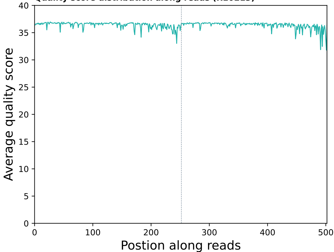
Quality score distribution along reads (R10213)
